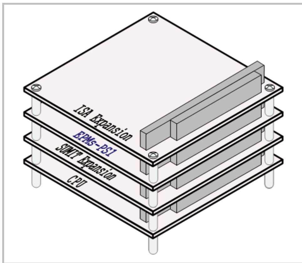
Figure 4. Stack Arrangement Example
