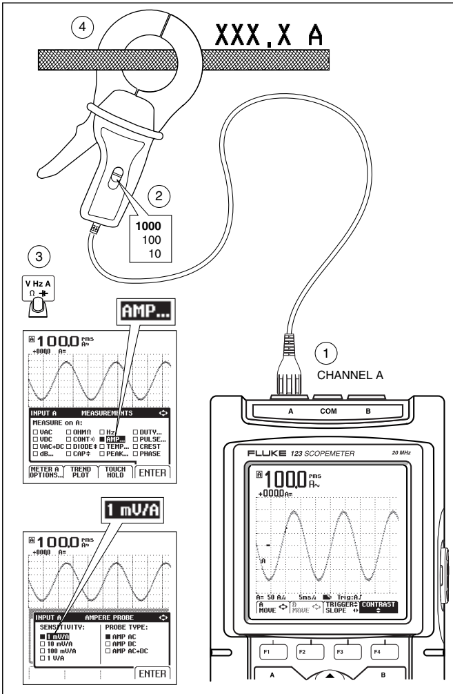
Figure 3. ScopeMeter Setups
