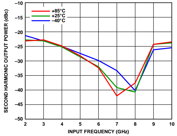
Figure 13. Second Harmonic Output Power ( P_2 ) vs. Input Frequency for Various Temperatures, Input Power = 10 dBm
