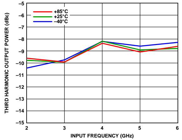
Figure 14. Third Harmonic Output Power ( P_3 ) vs. Input Frequency for Various Temperatures, Input Power = 10 dBm
