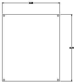
INNER PANEL
